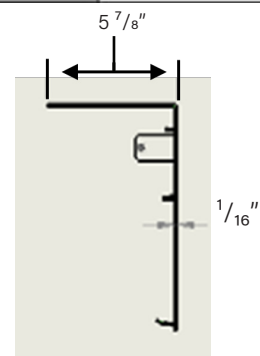
NFPA101 Bracket
