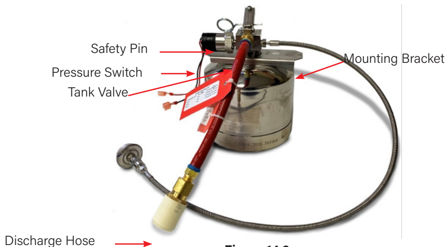
Figure 14.9 Extinguisher Tank Assembly
