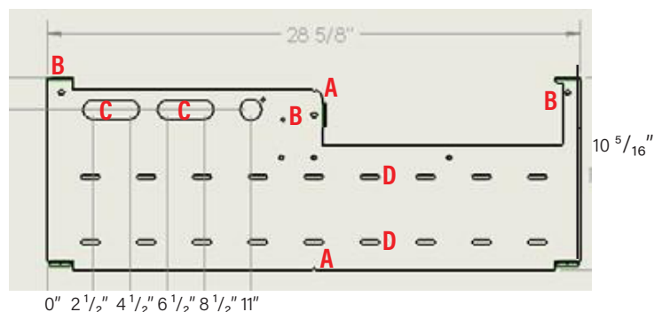
Mounting Bracket for D1000-F/R (non-NFPA101)
